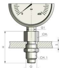
Tenuta tramite o-ring / O-ring sealing
