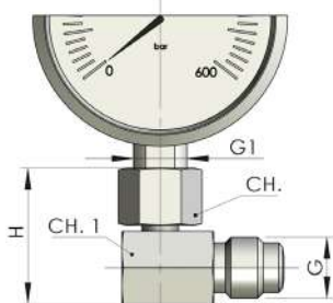
Tenuta tramite o-ring / O-ring sealing
